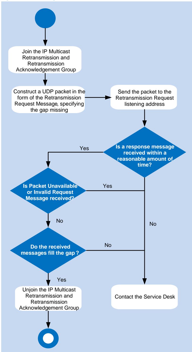
Figure 7 Processing of Line Level Retransmissions
