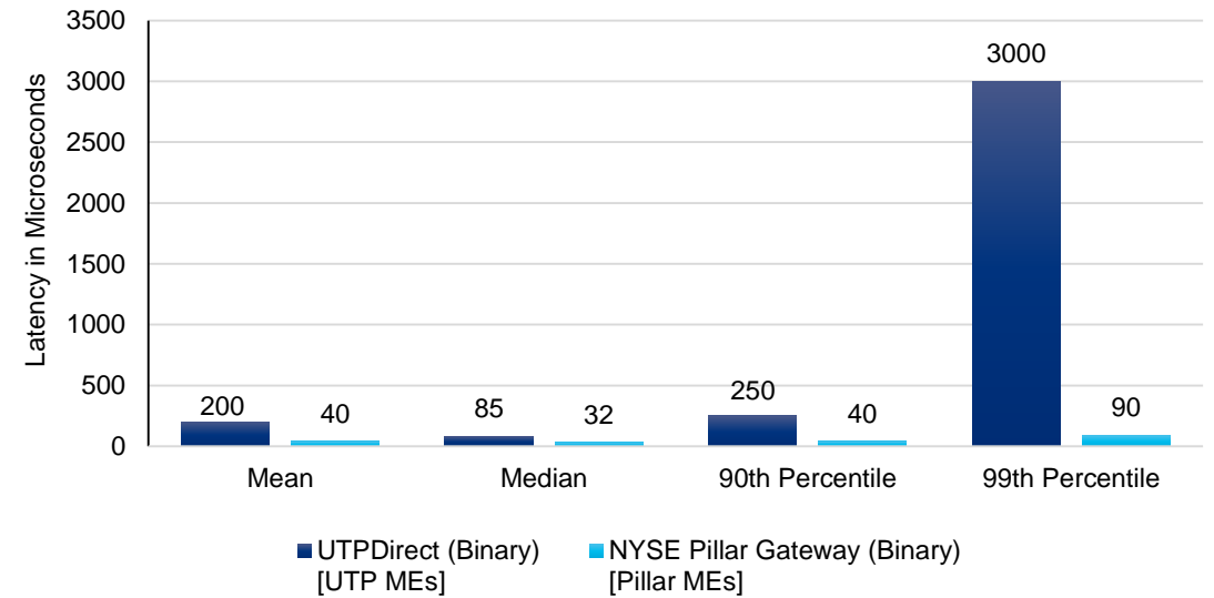
NYSE Tape A Projected Round-Trip Latency
